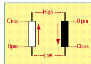
Candlestick Charts
